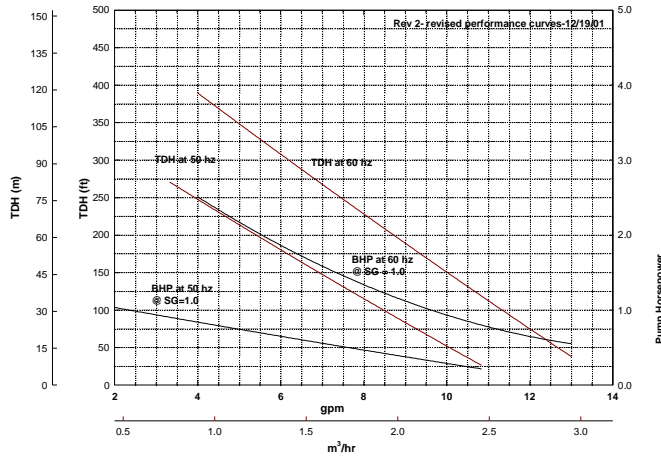
PT8 3450 & 2880 Curve
