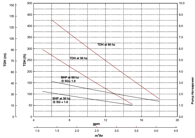
PT13 3450 & 2880 Curve
