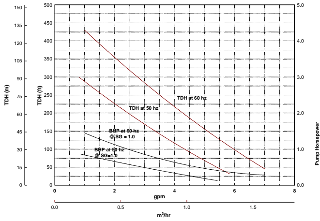
PT4 3450 & 2880 Curve
